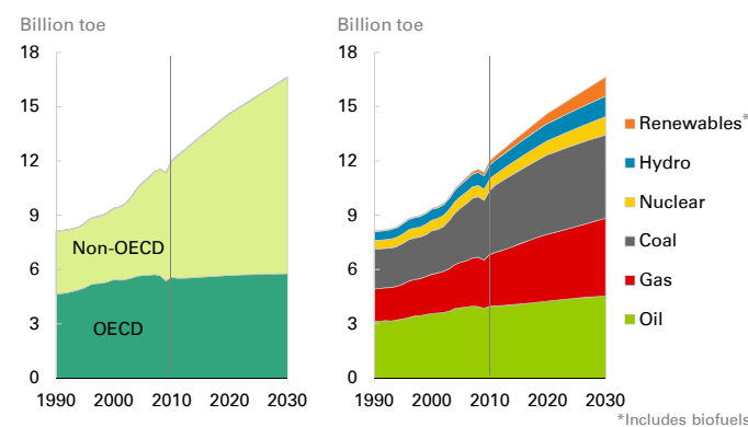
Energy consumption by region and fuel
