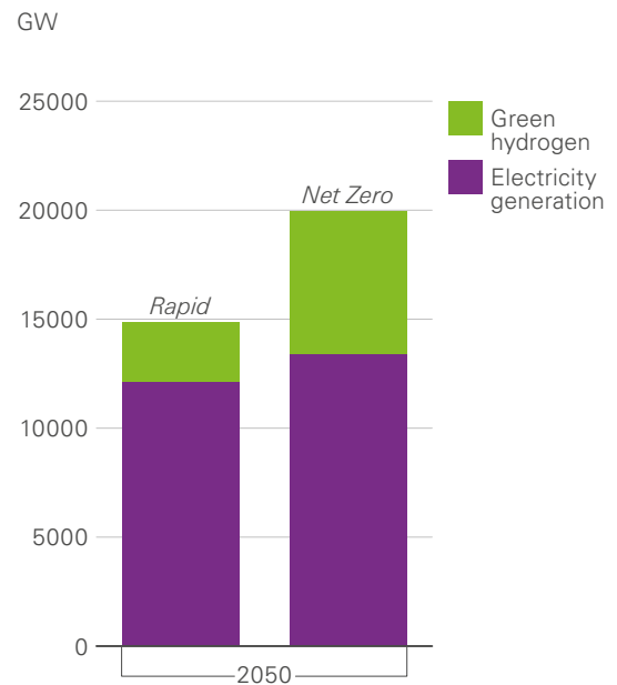
Installed capacity of wind and solar energy
