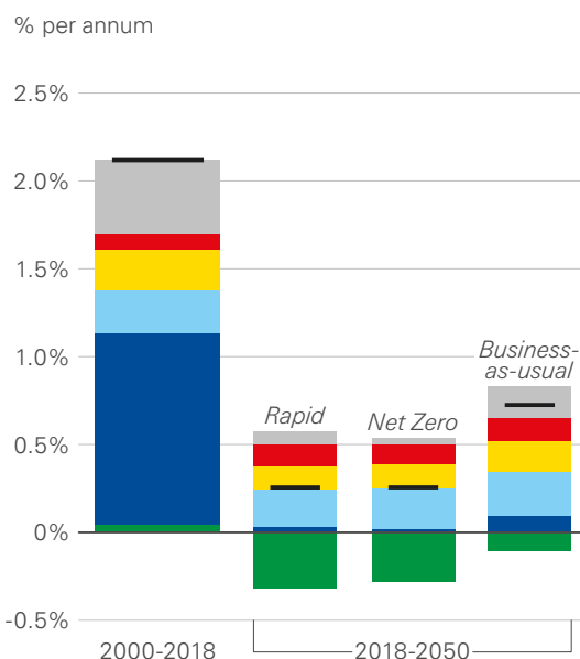
Primary energy growth and regional contributions
