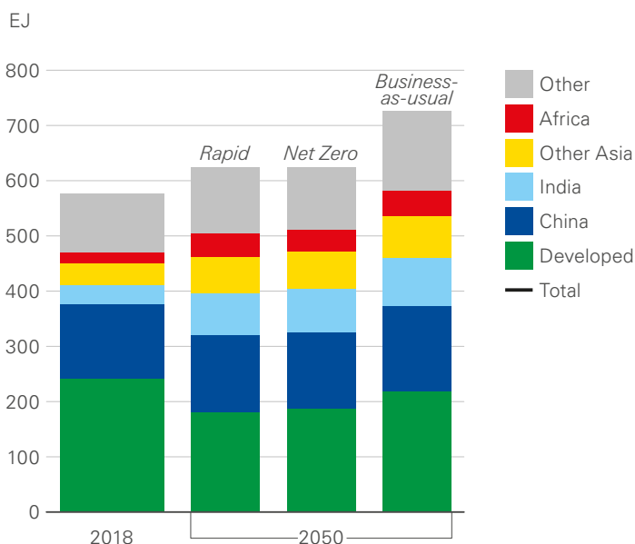
Primary energy consumption by region
