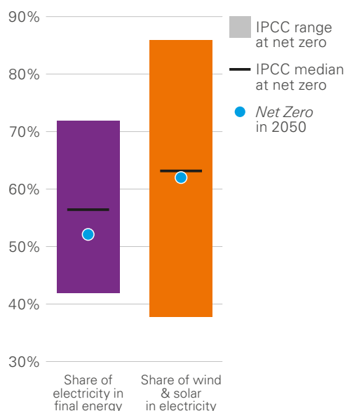
Shares of electricity, wind and solar in IPCC scenarios and Net Zero
