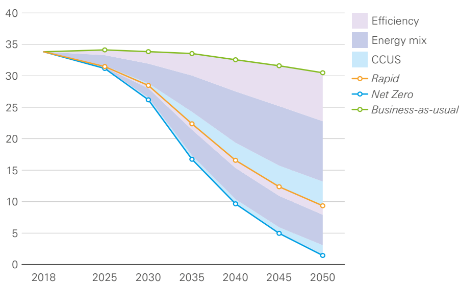
Carbon emissions from energy use
