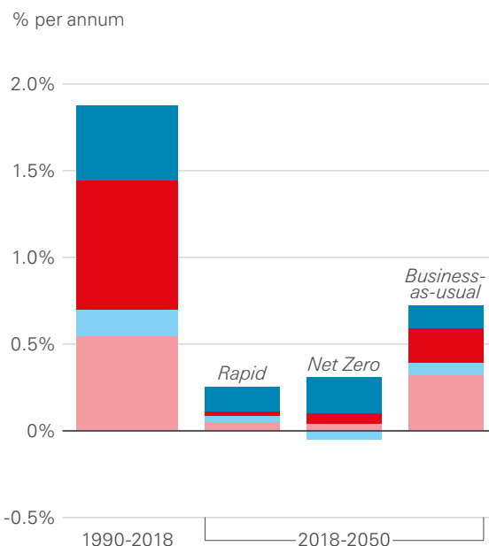
Annual demand growth and sector contributions
