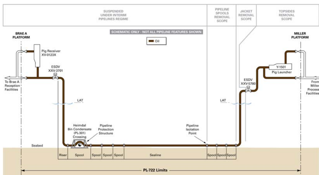
Figure 7.2: 18in Oil Export Pipeline (PL-722) Details
