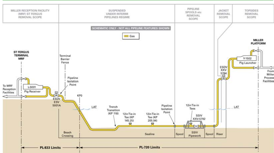
Figure 7.1: 30in Gas Export Pipeline (PL-720/PL-833) Details
