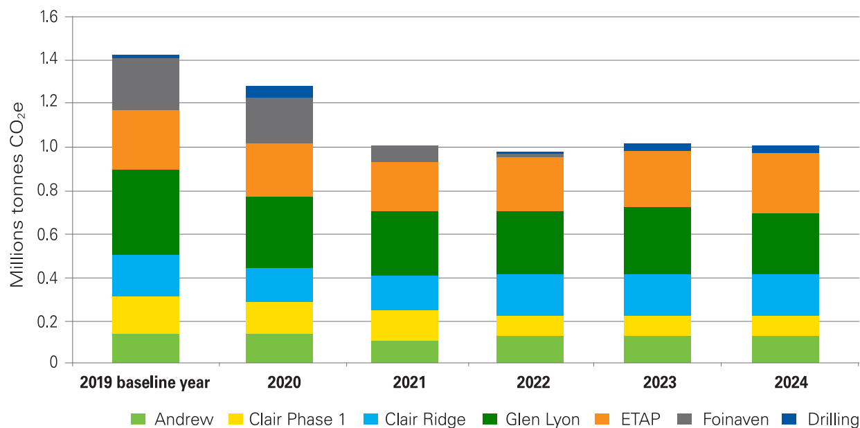
Figure 2: Total greenhouse gas emissions between 2019 and 2024.
