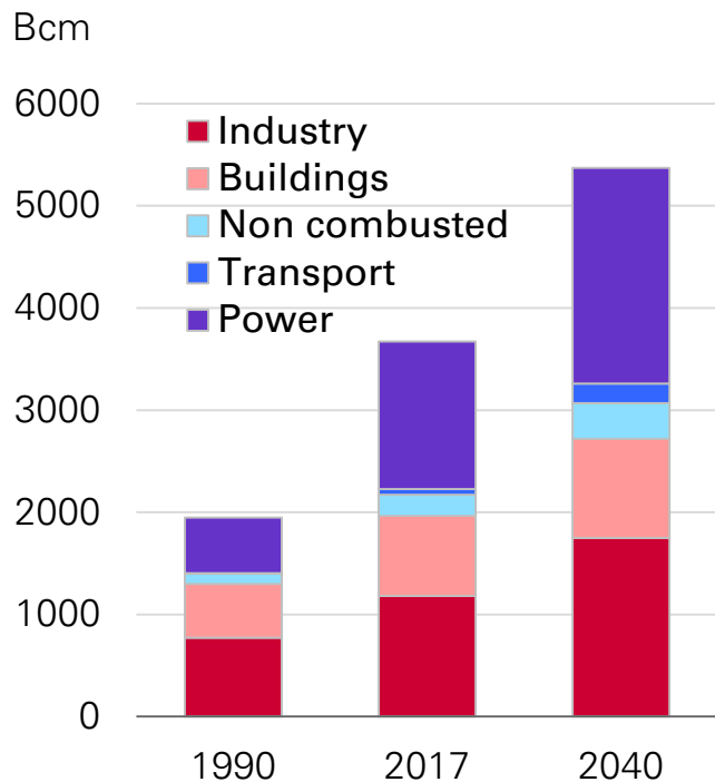
Gas consumption: By sector
